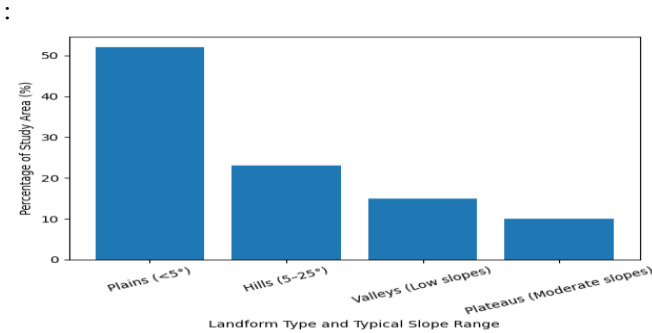
Figure 5a: Histogram illustrating slope distribution across plains, hills, valleys, and plateaus.
